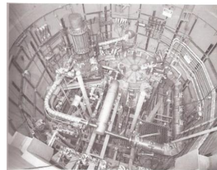
Figure 20. Top view of MSRE, the Molten Salt Reactor Experiment. (Courtesy of Oak Ridge National Laboratory.)
